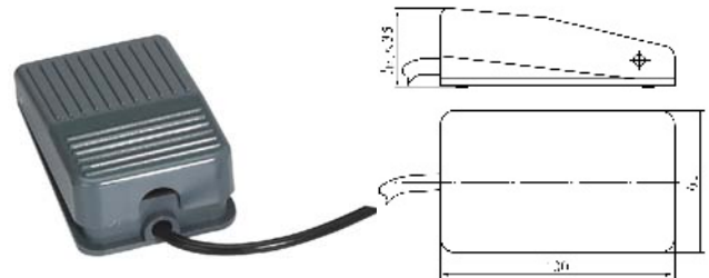
LJFS1-2(塑壳Plastic cover)
